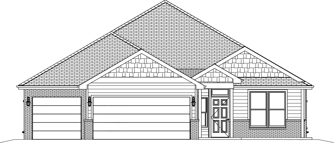
ELEVATION "A"
