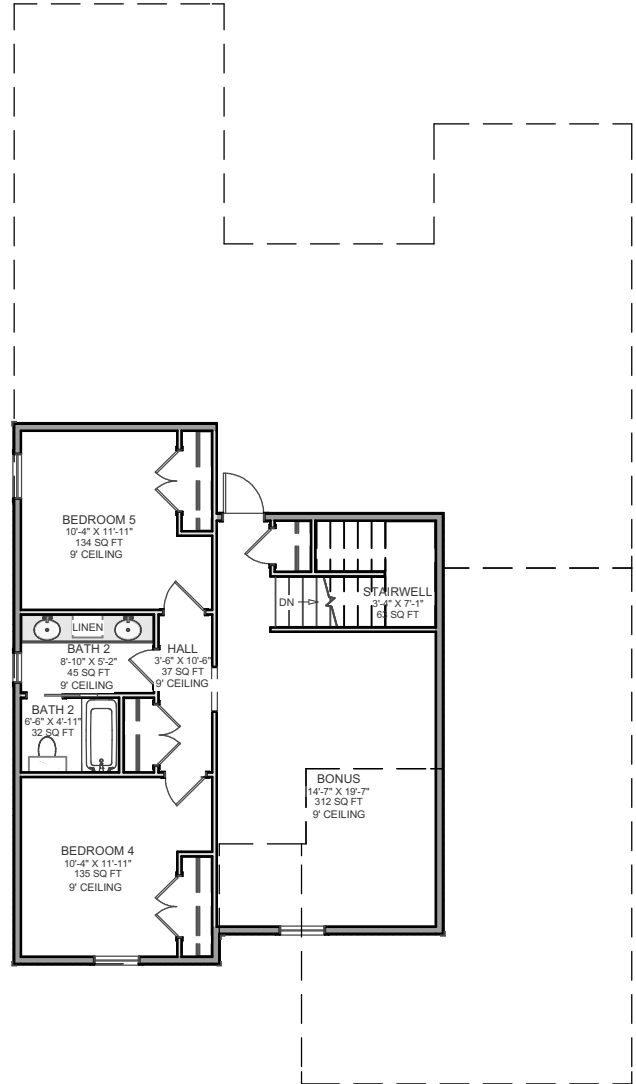
UPPER FLOOR
