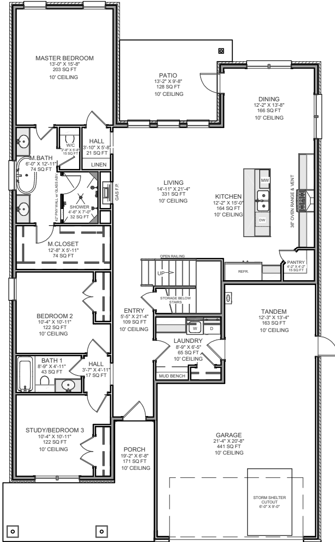
FIRST FLOOR
