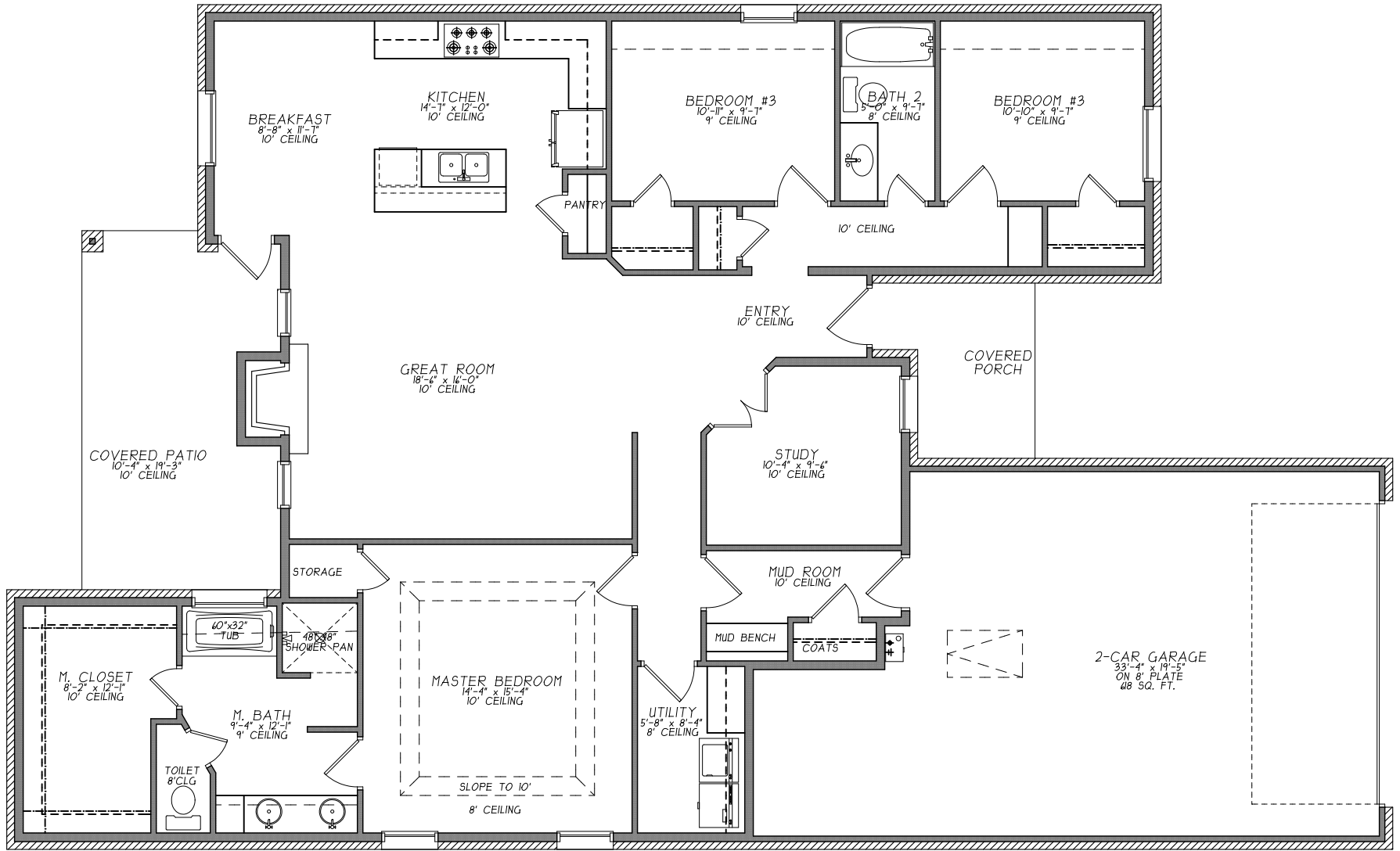
FLOOR PLAN
